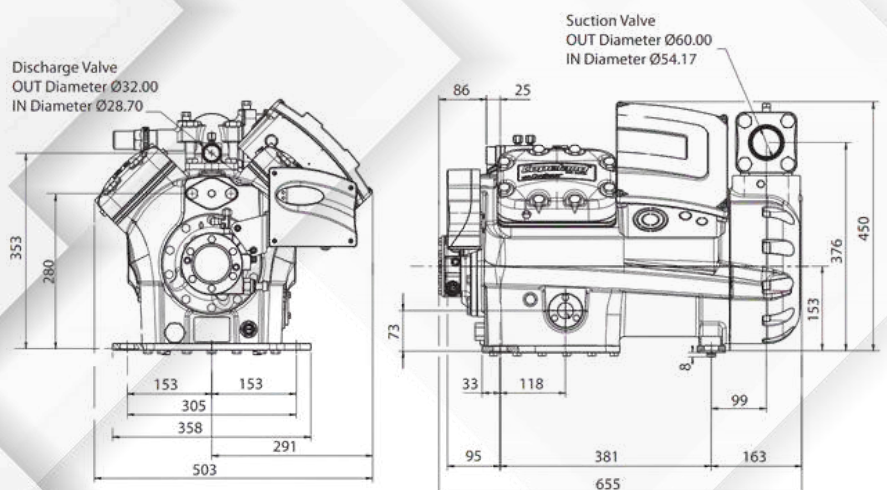
25HP : Model: 4MH-25X
