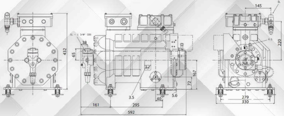
10 HP : Model: 3DC-100X
