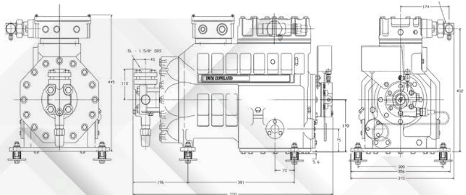
25HP : Model: 4MH-25X
